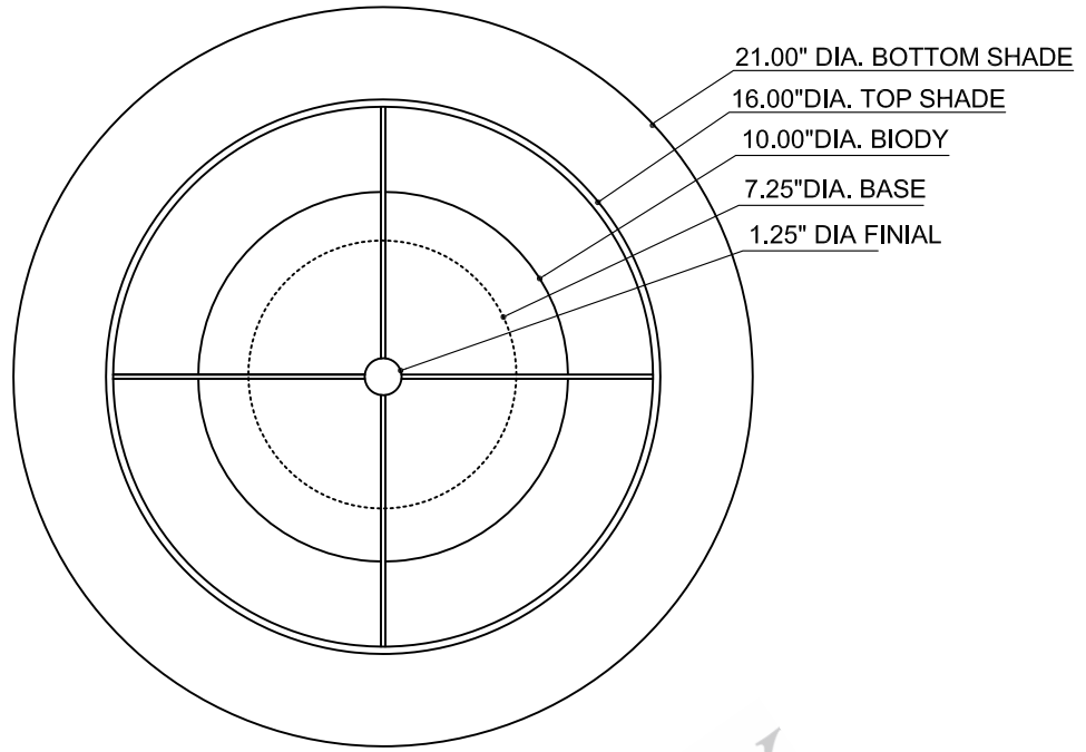
TOP VIEW
